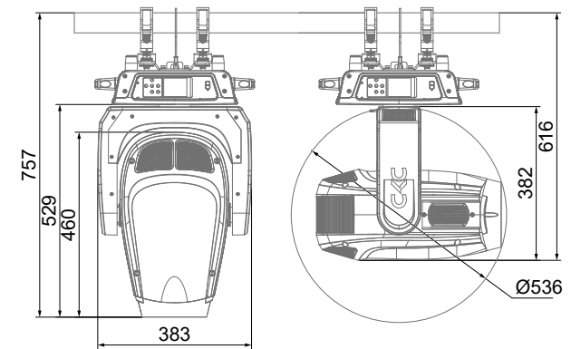
Integrated clamp installation
