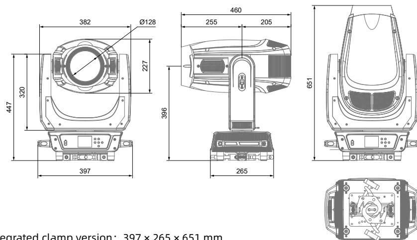
Integrated clamp version: 397 × 265 × 651 mm
