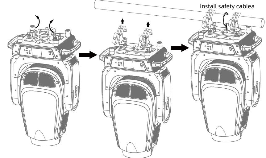
Integrated clamp installation
