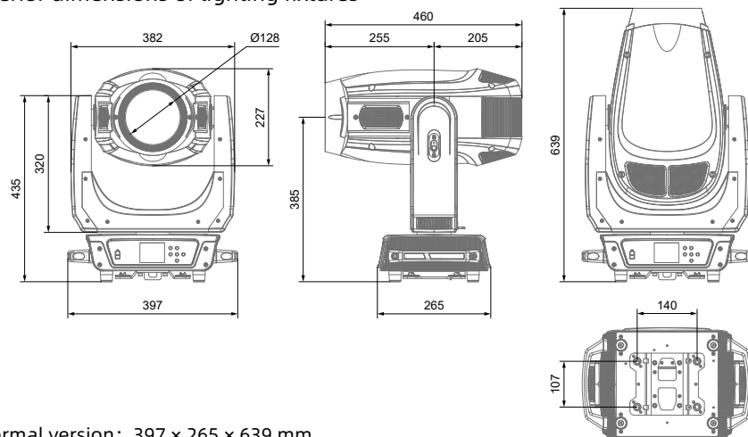
Normal version: 397 × 265 × 639 mm
